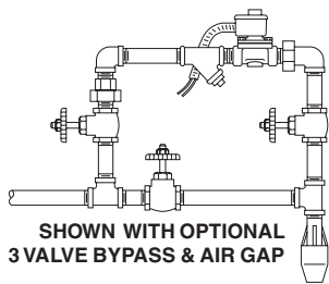
FIGURE A Three-valve Make-up Bypass
