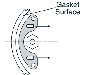
Figure 5 For traps 214, 215, 216, 314 and larger 814, 815 and 816.
